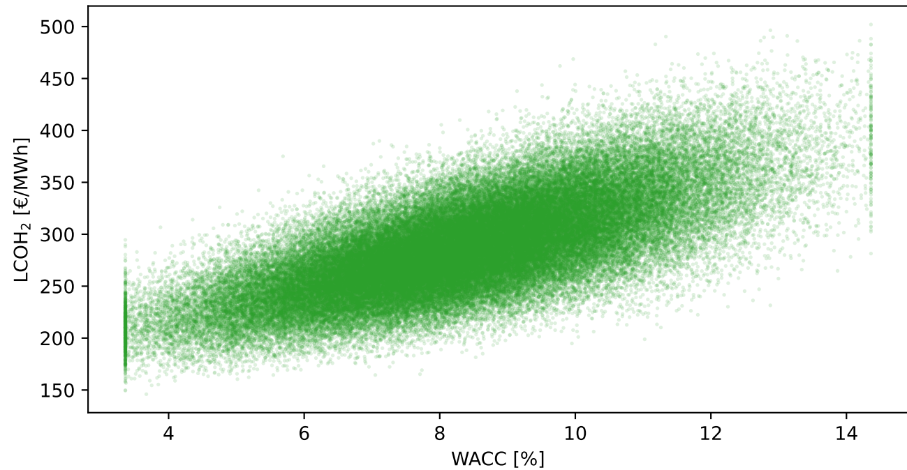
LCOH 2 vs WACC
